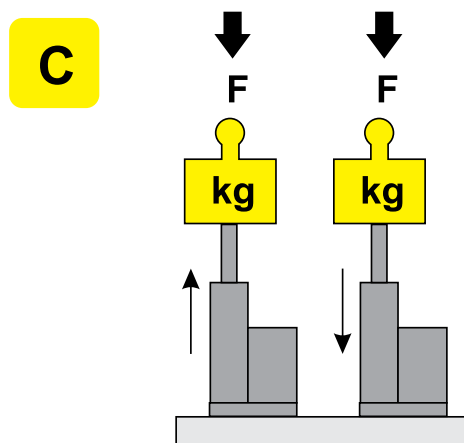
Configuration C: load is always acting to drive the piston rod into the actuator.
