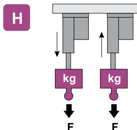
Configuration H: load is always acting to draw the piston rod out of the actuator
