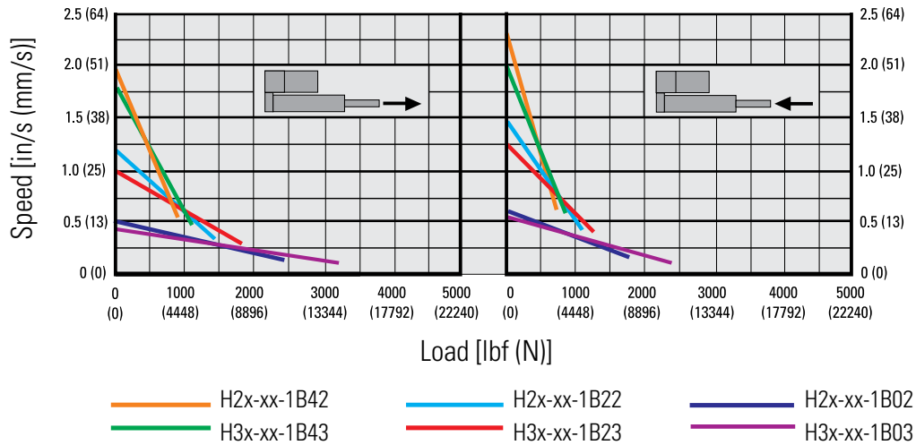
Motor Type 2 - Load vs. Speed @ Extension / Retraction
