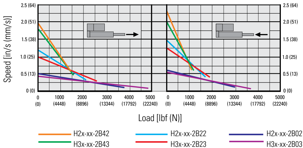
Motor Type 3 - Load vs. Speed @ Extension / Retraction
